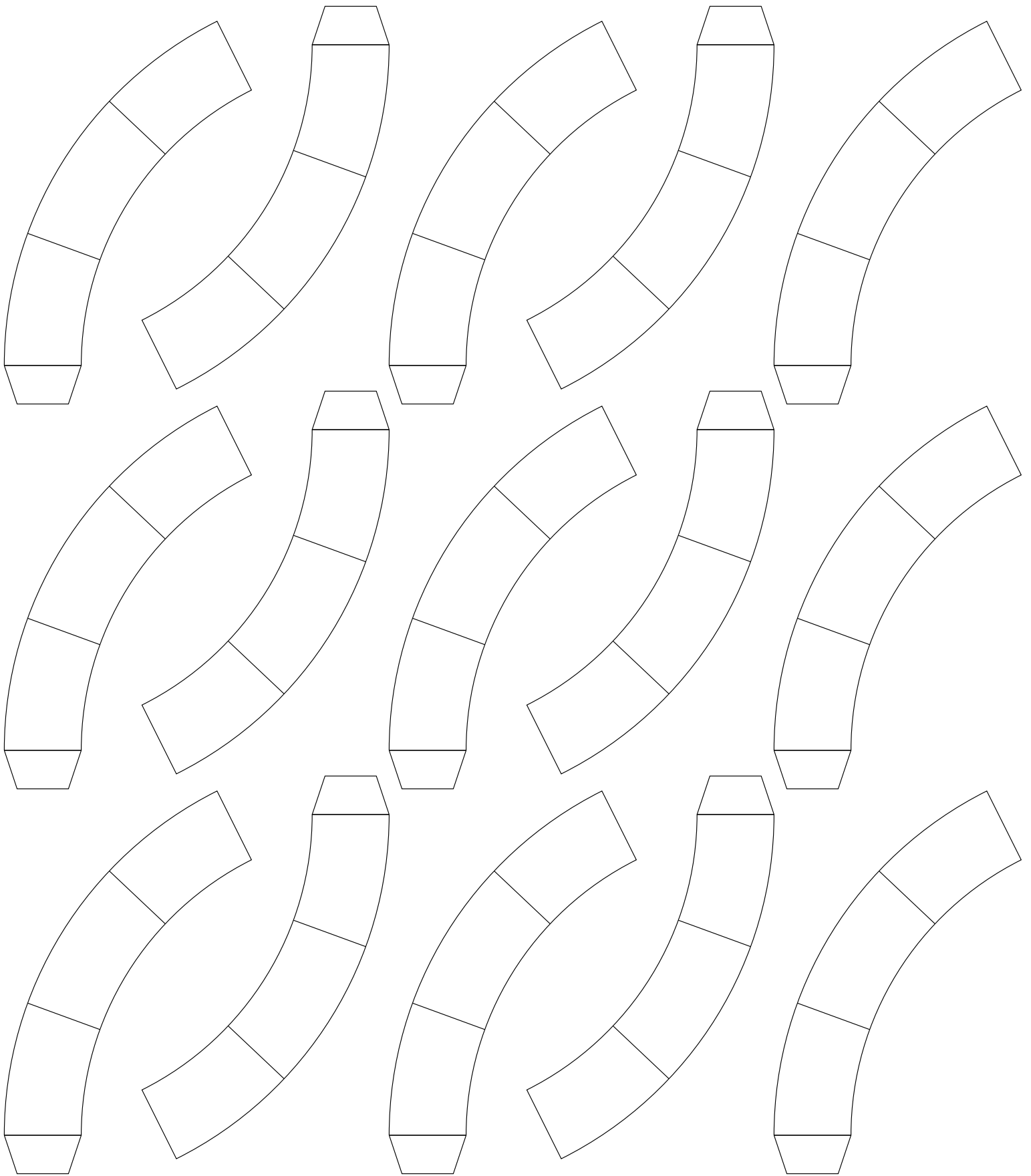
truncated icosahedron, pentagonal subtriangles, 20.1 23.3 20.1
