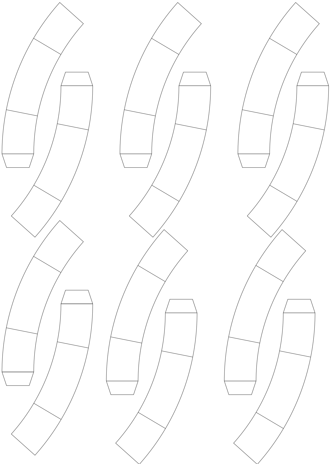
truncated dodecahedron 11.2 19.4 11.2
