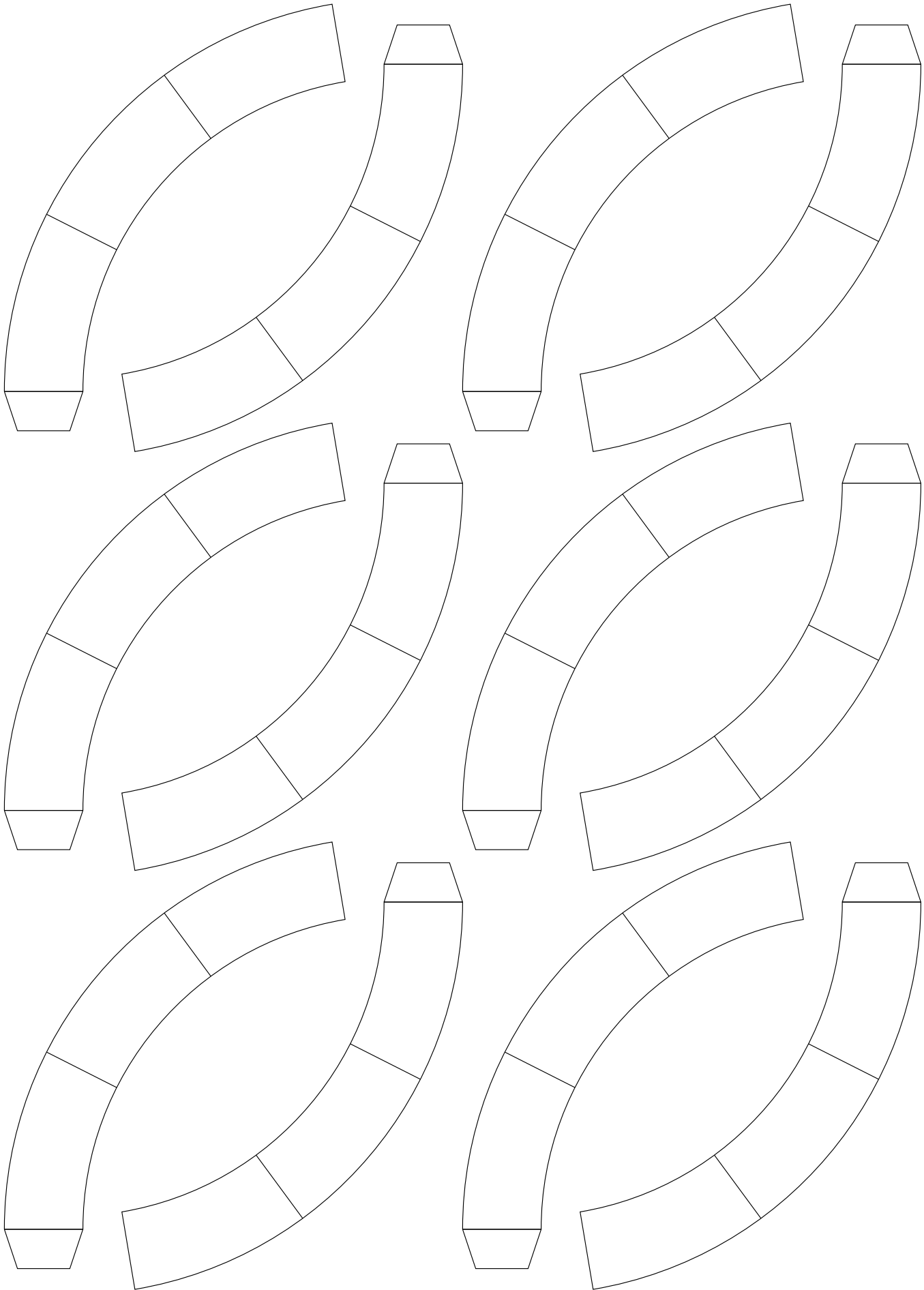
geodesic snub dodecahedron 26.8 26.8 26.8
